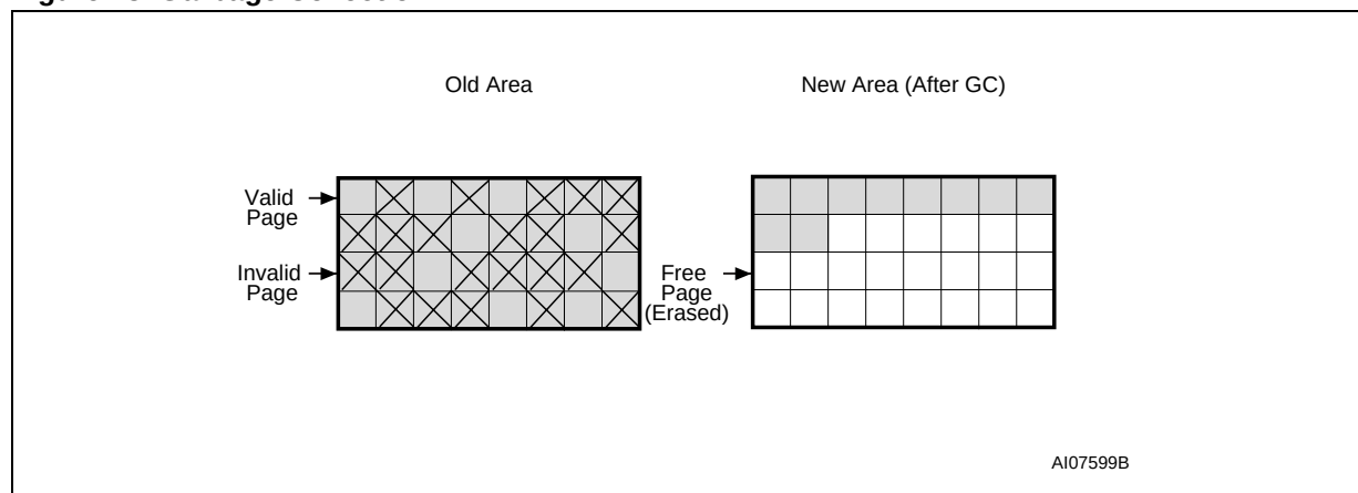
Figure 23. Garbage Collection
