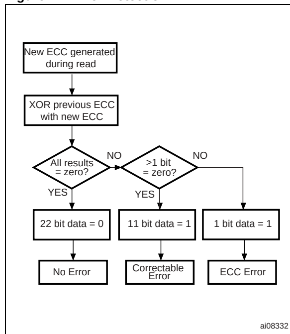
Figure 24. Error Detection
