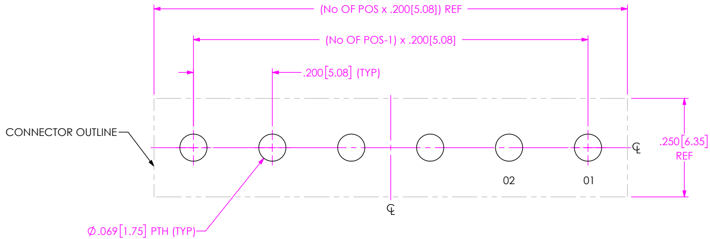
FIG 1 HPM-XX-XX-XX-S SHOWN (FOR -S & -S-RA OPTIONS)
