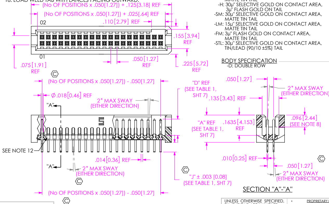
FIG 1 THROUGH HOLE -01, -03, -11, -13, -21, -23, -31
