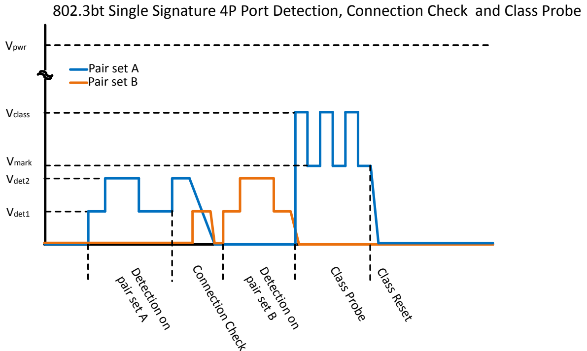
Figure 2.4. Semi-Auto DET/CC/CLASS 4-Pair Single-Signature Waveform
