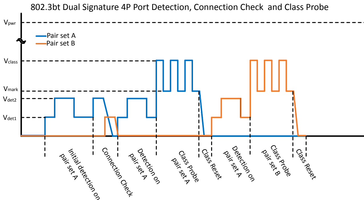
Figure 2.5. Semi-Auto DET/CC/CLASS 4-Pair Dual-Signature Waveform
