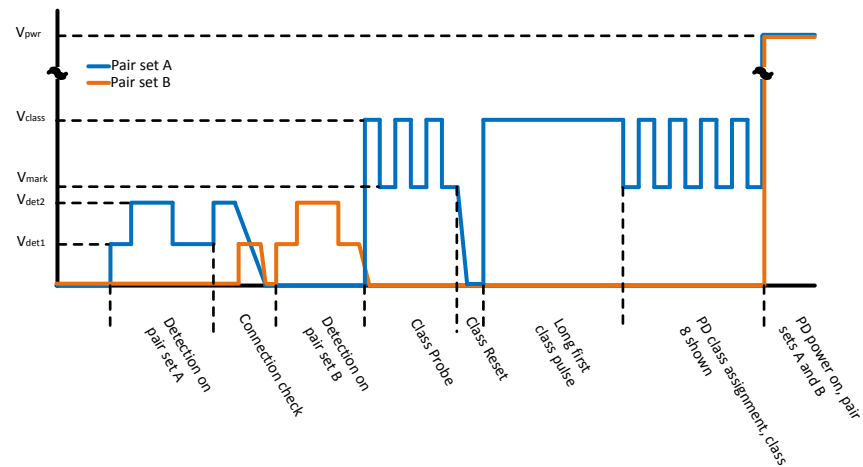
Figure 2.7. 4P Single-Signature Port Detection Waveform
