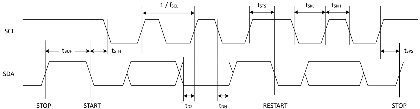
Figure 5.1. I²C Bus Interface Timing
