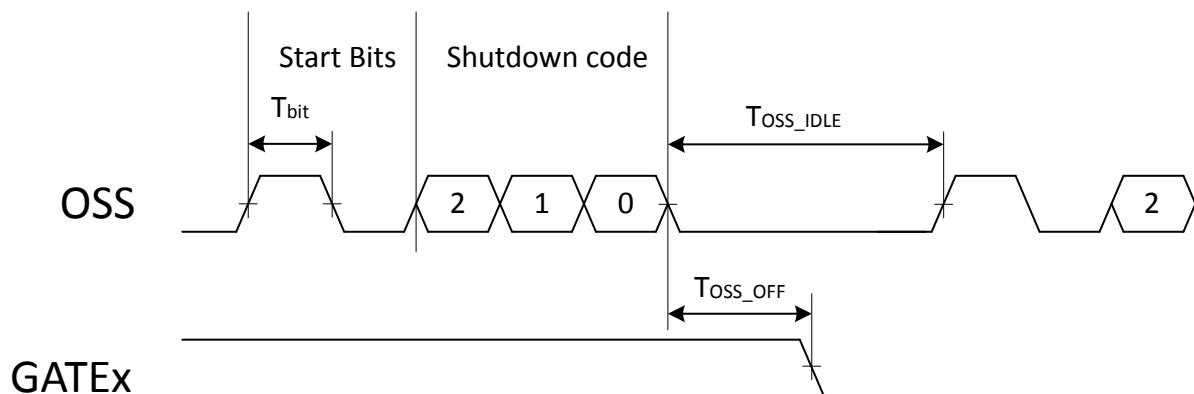
Figure 2.10. OSS Pin in Multi-Bit Mode
