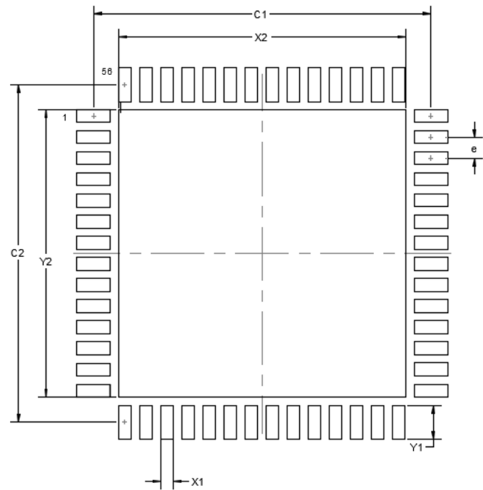
Figure 8.1. Si3474 Recommended Land Pattern
