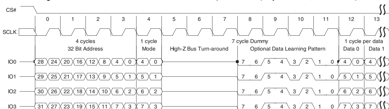
Figure 10.52 Continuous DDR Quad I/O Read Subsequent Access (4-byte Address, EHPLC=01b)
