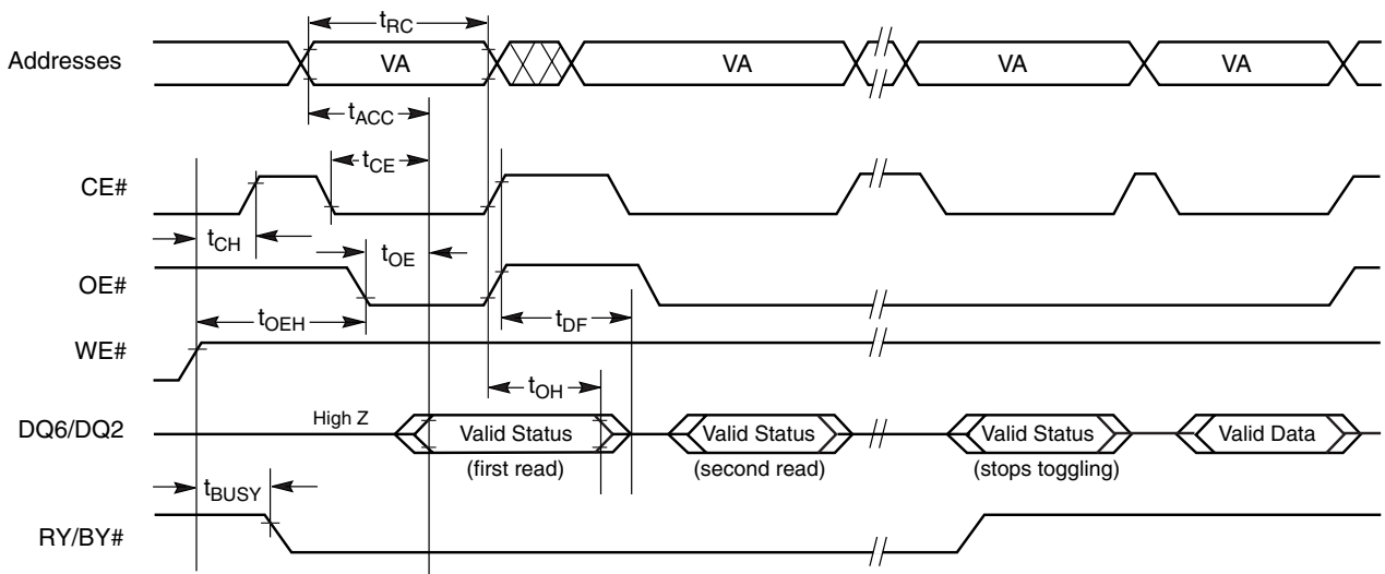
Figure 21. Toggle Bit Timings (During Embedded Algorithms)
