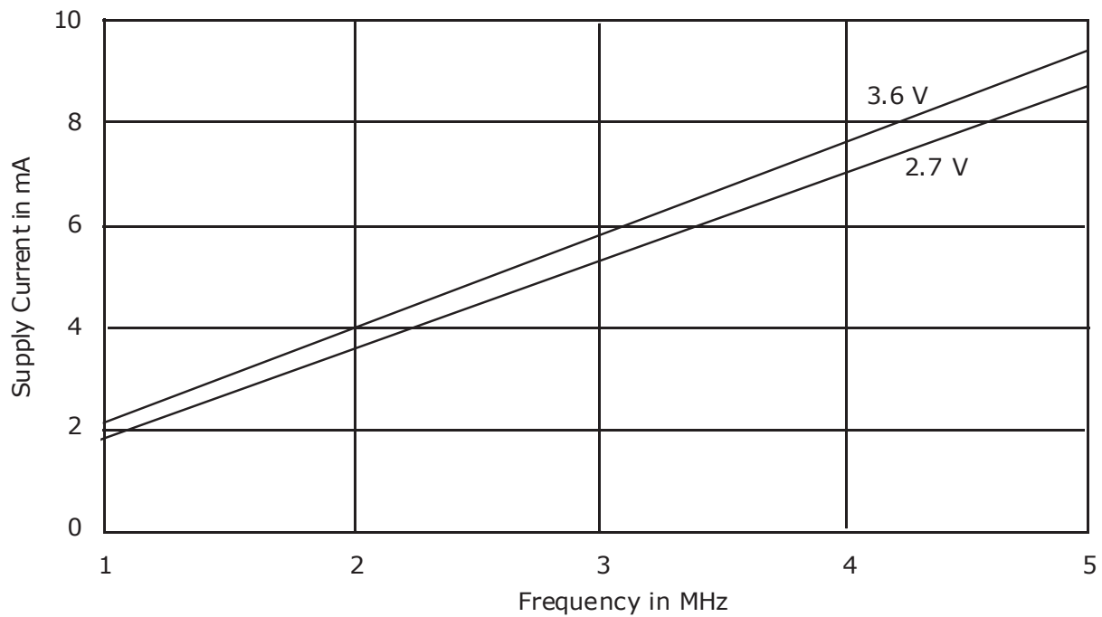
Figure 11. Typical I_{CC1} vs. Frequency
