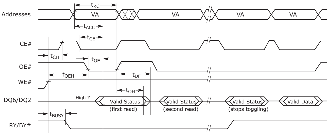
Figure 21. Data# Polling Timings (During Embedded Algorithms)
