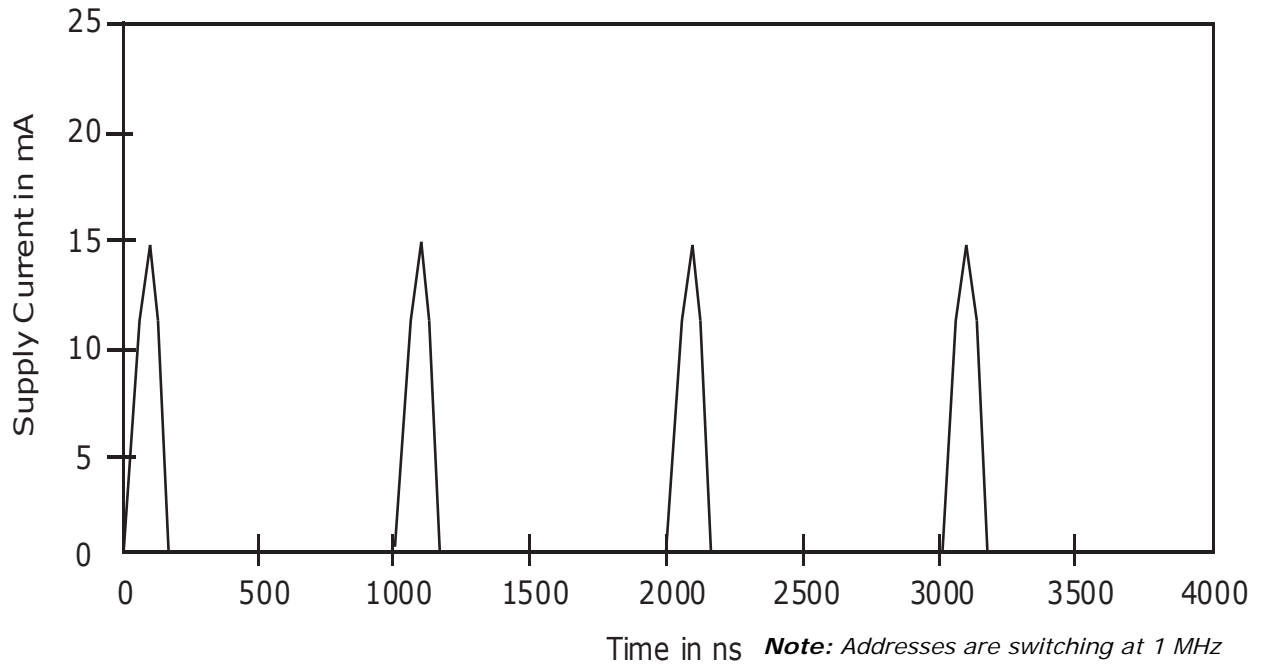
Figure 10. I_{CC1} Current vs. Time (Showing Active and Automate)
