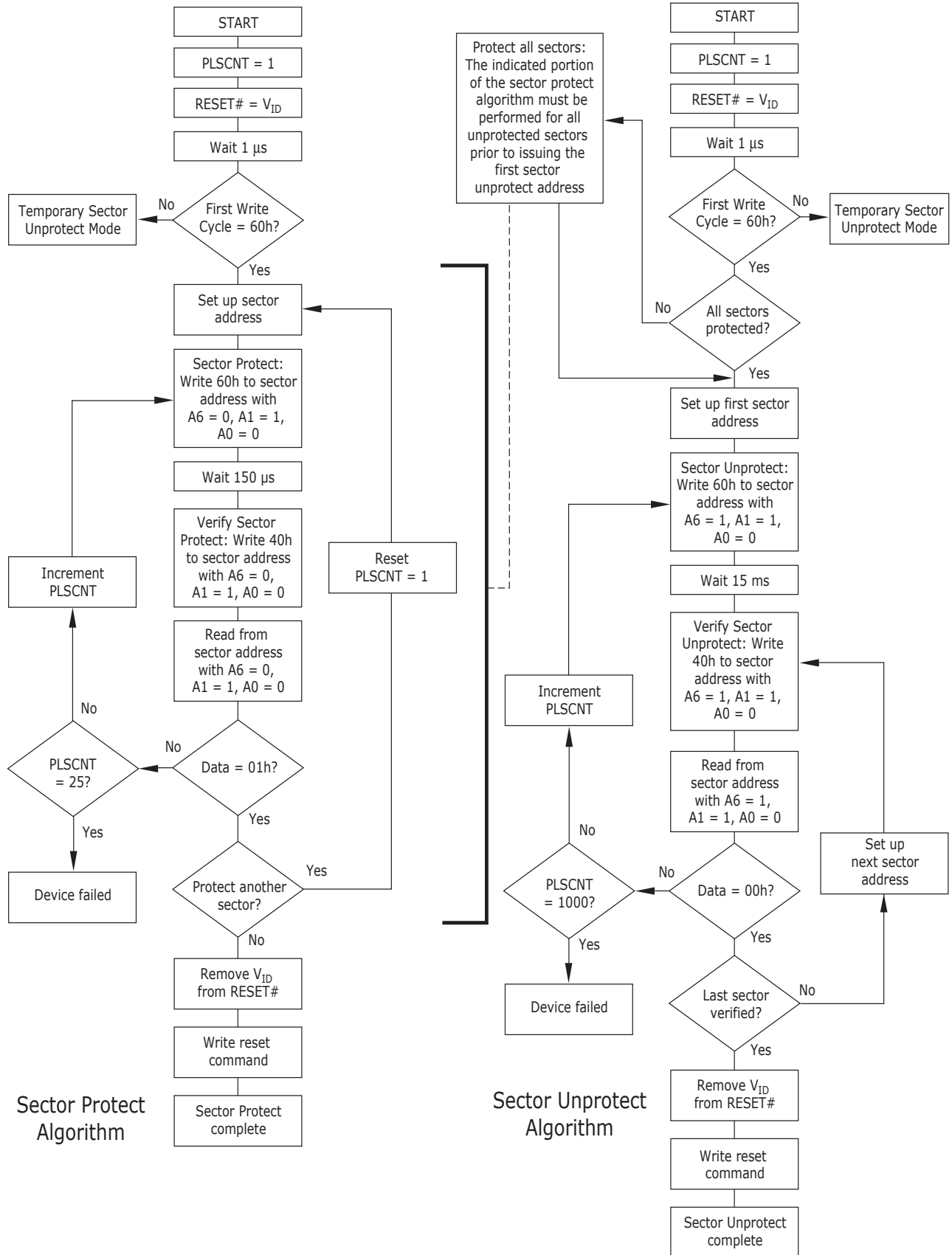
Figure 2. In-System Sector Protect/Unprotect Algorithms
