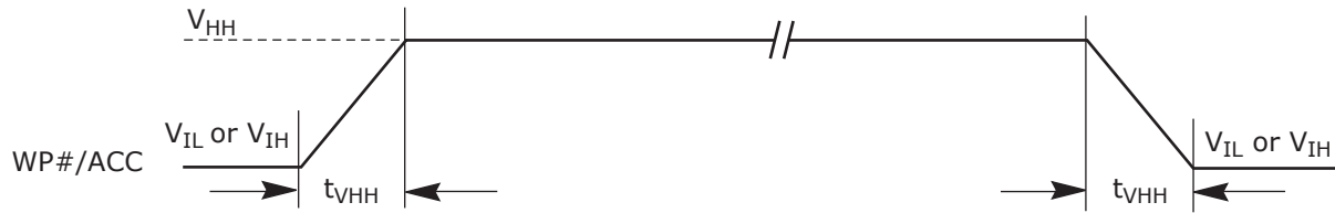
Figure 25. Accelerated Program Timing Diagram
