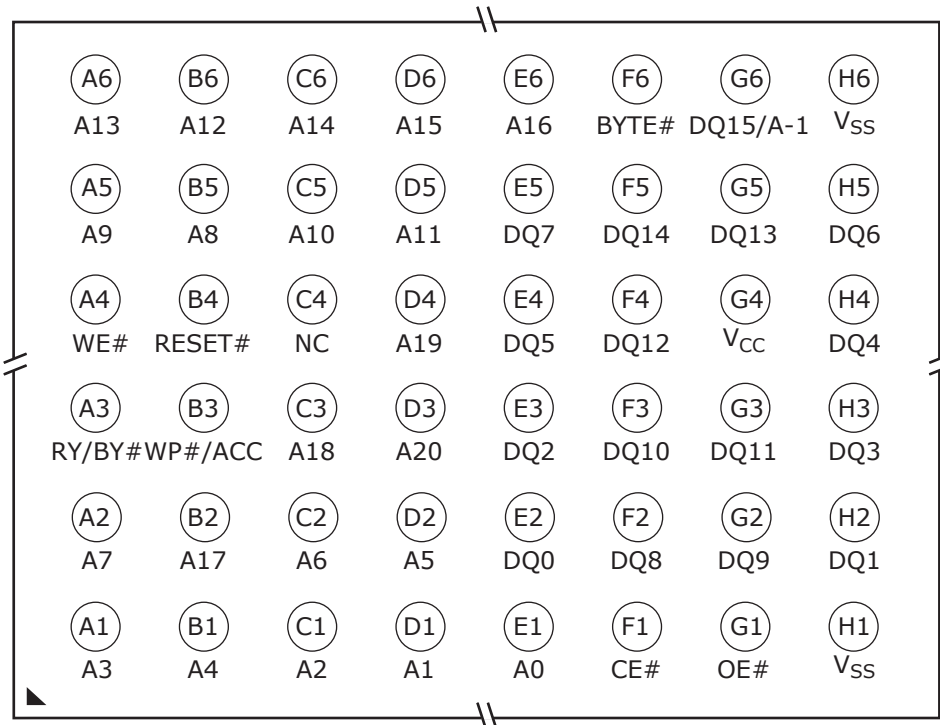
48-ball FBGA Top view balls facing down
