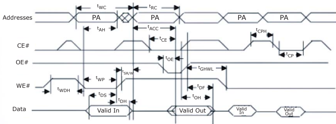
Figure 20. Back to Back Read/Write Cycle Timing
