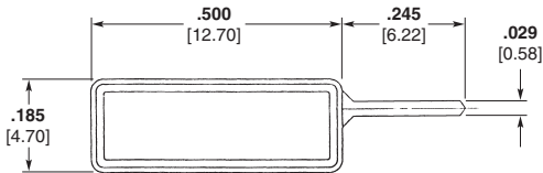
Polarizing Key 1-1437023-2
