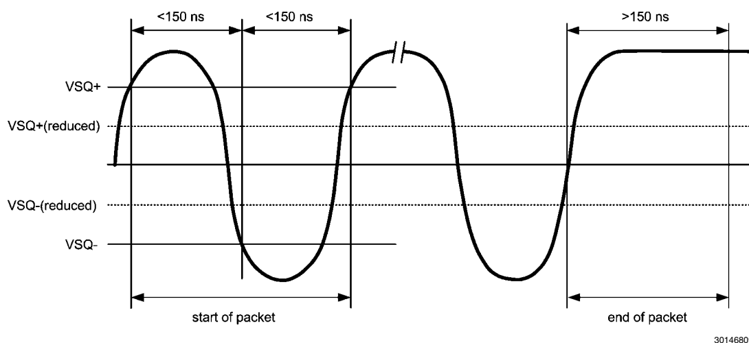
FIGURE 7. 10BASE-T Twisted Pair Smart Squelch Operation
