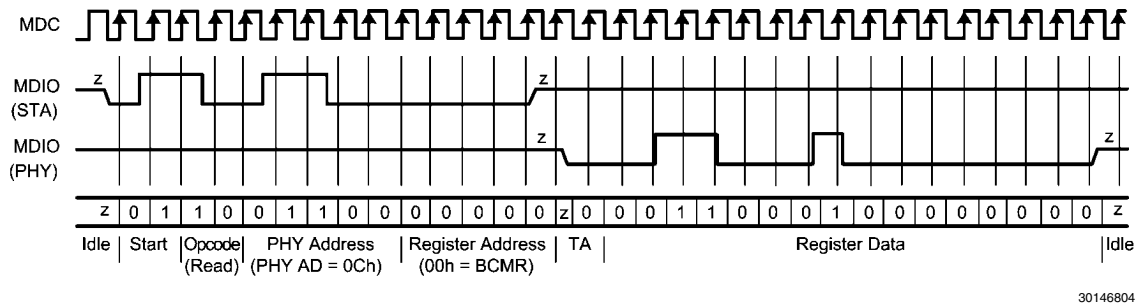
FIGURE 3. Typical MDC/MDIO Read Operation
