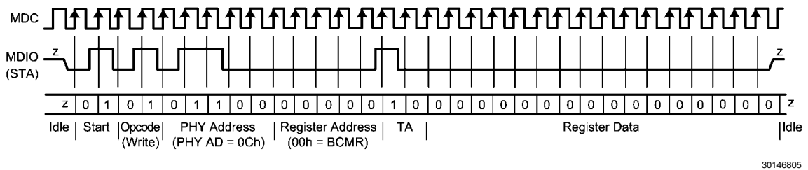
FIGURE 4. Typical MDC/MDIO Write Operation
