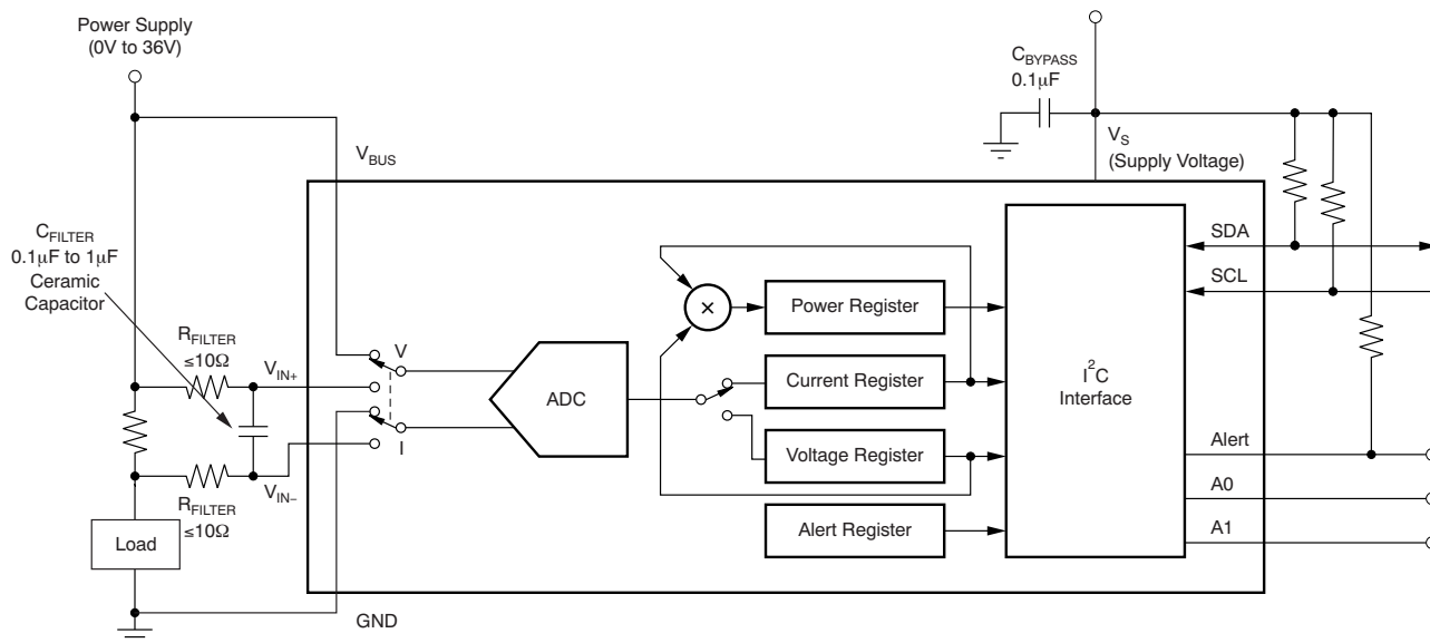
Figure 22. INA226 with Input Filtering
