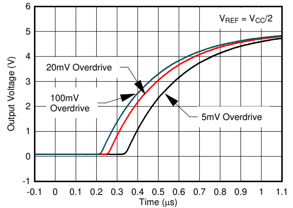
Figure 5-32. Response Time for Various Overdrives, Low-to-High Transition
