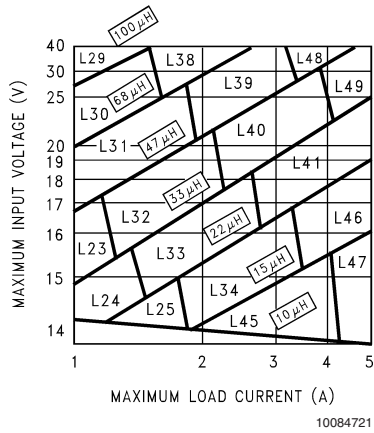
FIGURE 5. LM2679-12
