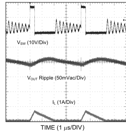
Discontinuous Mode Operation ( V_{OUT} = 3.3V , 0.15A Loaded)
