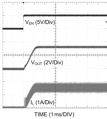
Enable Transient ( V_{OUT} = 3.3V , 1.5A Loaded)
