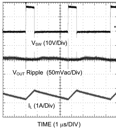
Continuous Mode Operation ( V_{OUT} = 3.3V , 1.5A Loaded)
