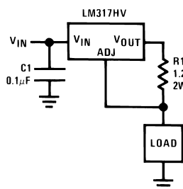
Figure 28. 1A Current Regulator
