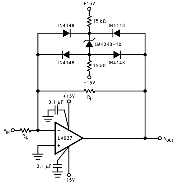
Figure 9. Bounded amplifier reduces saturation-induced delays and can prevent succeeding stage damage. Nominal clamping voltage is \pm 11.5V (LM4040's reverse breakdown voltage +2 diode V_F ).
