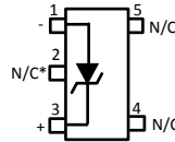
Figure 3. SC70 NS Package (Top View)
