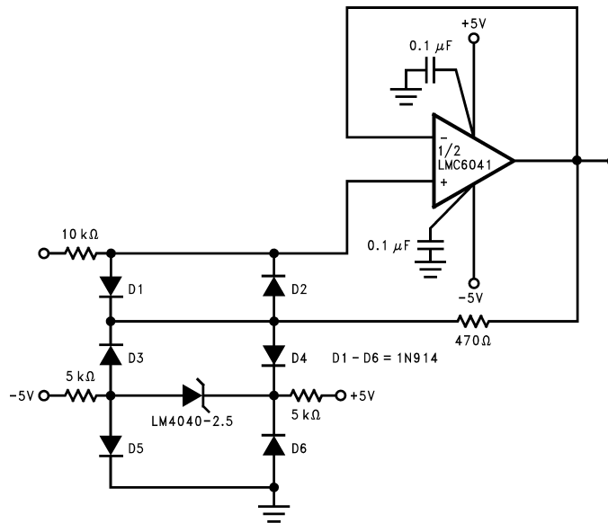
Figure 10. Protecting Op Amp input. The bounding voltage is \pm 4V with the LM4040-2.5 (LM4040's reverse breakdown voltage + 3 diode V_F ).
