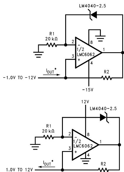
Figure 12. Precision 1 μA to 1 mA Current Sources
