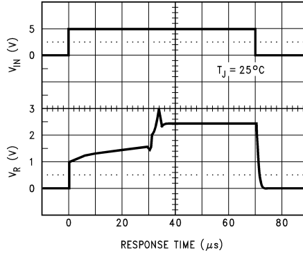
Figure 5. LM4040-5.0 R_S = 30k
