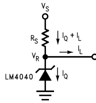
Figure 7. Shunt Regulator
