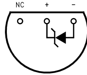
Figure 2. TO-92 NS Package(Bottom View)
