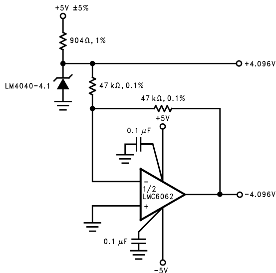
Figure 11. Precision ±4.096V Reference
