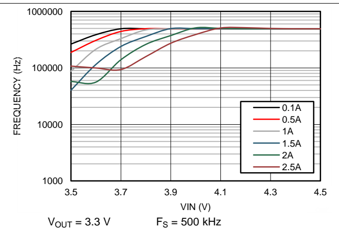
Figure 62. Frequency vs VIN
