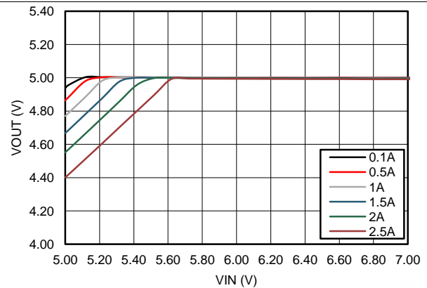
V_{OUT} = 5\text{ V} F_S = 1\text{ MHz}
