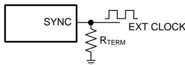
Figure 42. Frequency Synchronization
