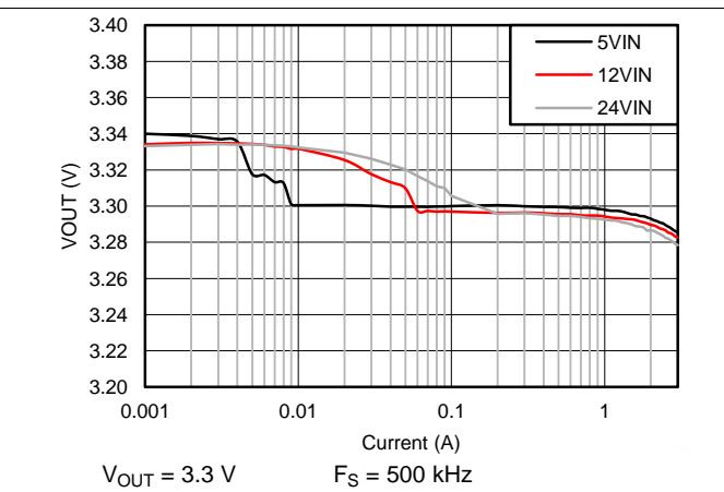
Figure 64. Output Voltage Regulation
