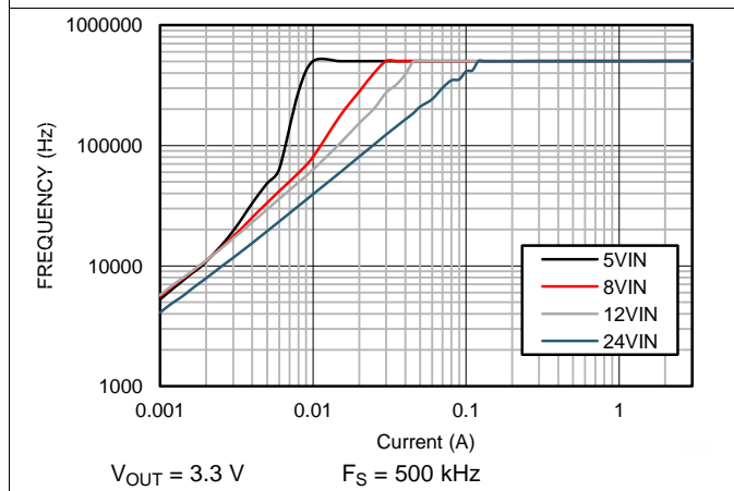
Figure 63. Frequency vs Load
