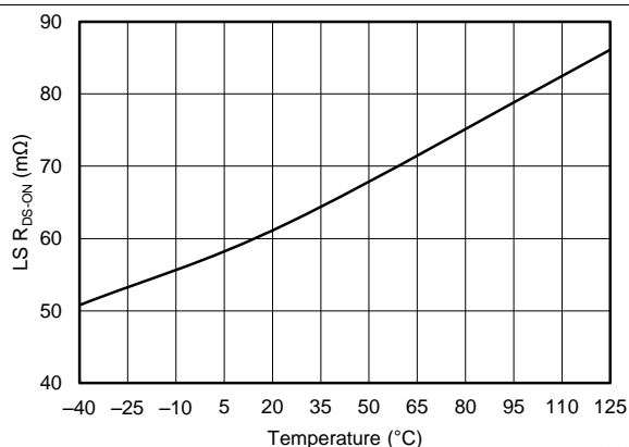
Figure 24. Low-Side FET On Resistance vs Junction Temperature
