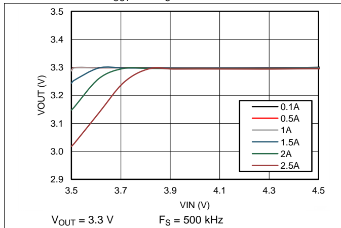
Figure 61. Dropout Curve
