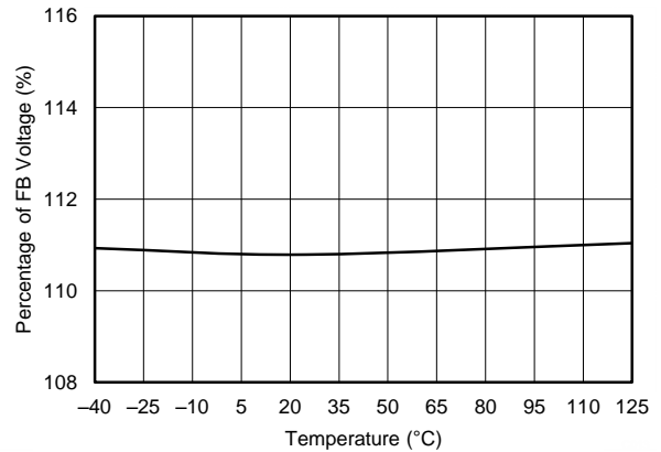
Figure 28. PGOOD OVP Rising Threshold vs Junction Temperature
