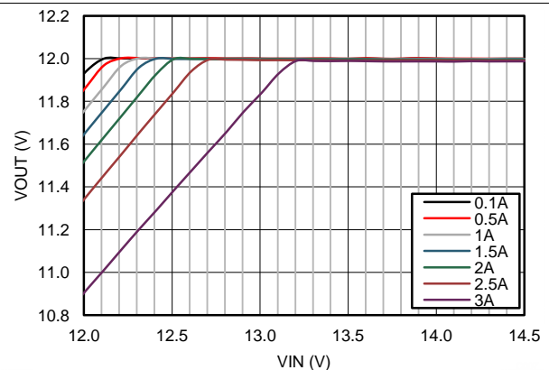
V_{OUT} = 12\text{ V} F_S = 500\text{ kHz}
