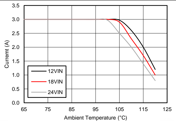
V_{OUT} = 1\text{ V} F_S = 500\text{ kHz} \theta_{JA} = 20^{\circ}\text{C/W}
