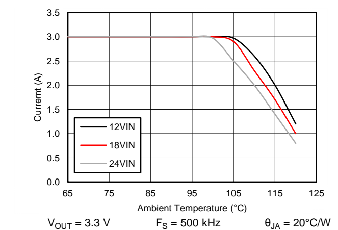
Figure 66. Derating Curve
