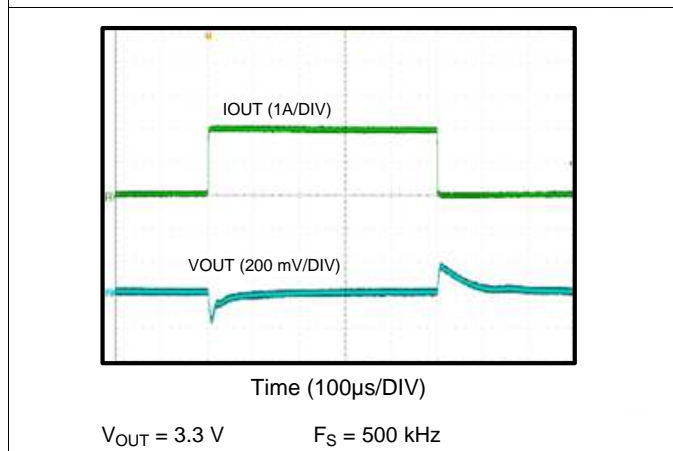
Figure 65. Load Transient 0.1A to 2A
