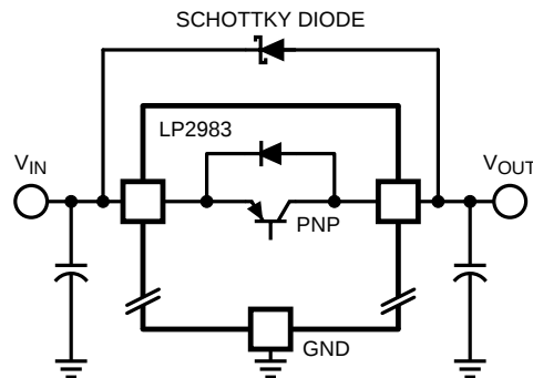
Figure 24. Adding External Schottky Diode Protection
