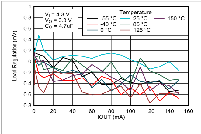
Figure 6-7. Output Regulation vs Load Current for New Chip
