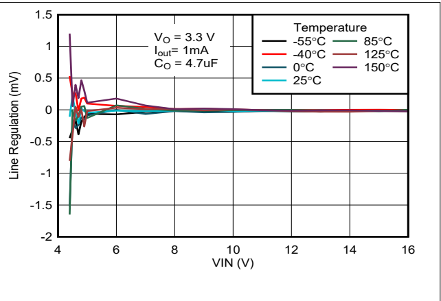
Figure 6-8. Output Regulation vs Input Voltage for New Chip
