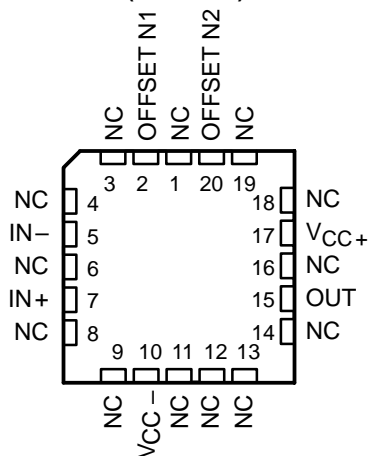
FK PACKAGE
