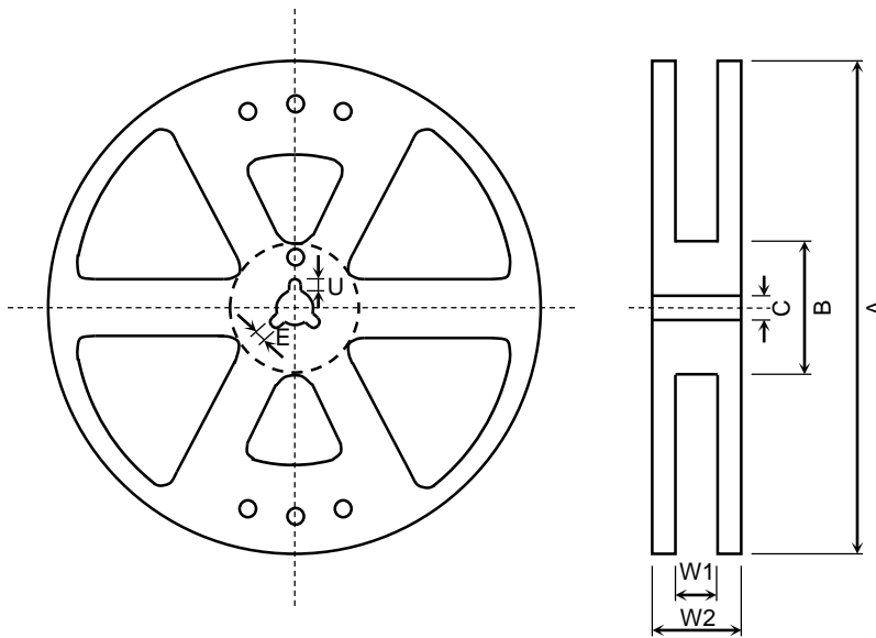
Figure 3.6.1 Reel Dimensions
