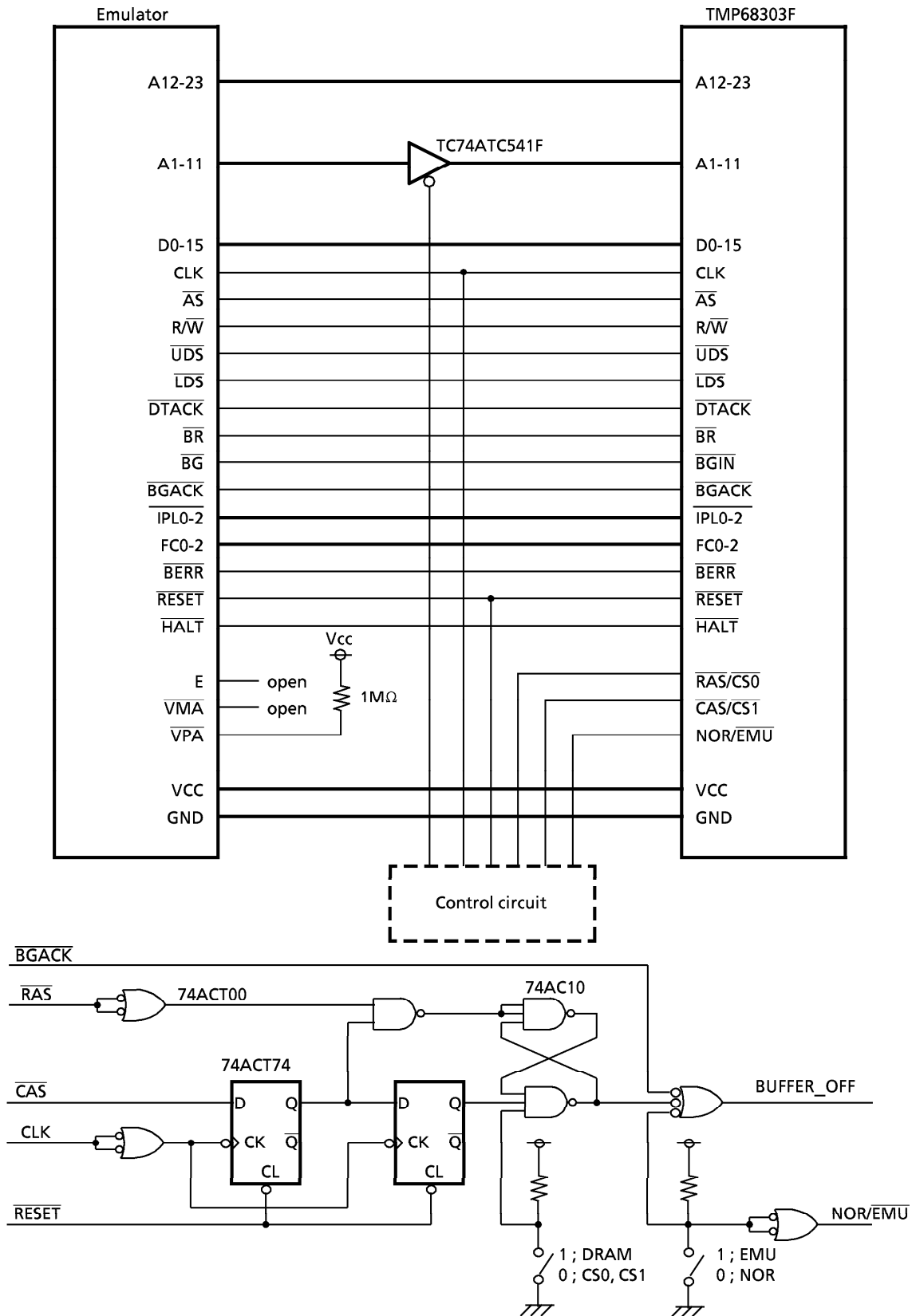
Figure 14.7 Control Circuits
