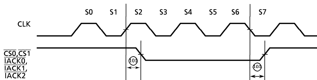
Figure 13.5 \overline{CS} , \overline{IACK} , \overline{DACK} Timing
