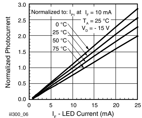
Fig. 6 - Normalized Servo Photocurrent vs. LED Current and Temperature
