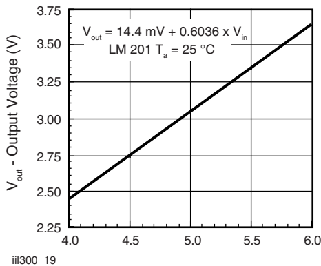
Fig. 16 - Transfer Gain
