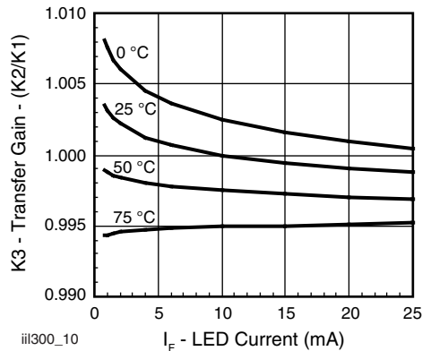
Fig. 9 - Transfer Gain vs. LED Current and Temperature
