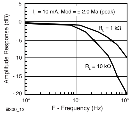
Fig. 11 - Amplitude Response vs. Frequency
