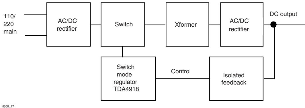
Fig. 5 - Switching Mode Power Supply
