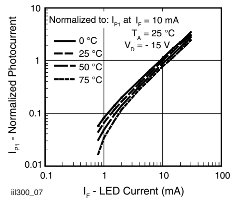
Fig. 7 - Normalized Servo Photocurrent vs. LED Current and Temperature
