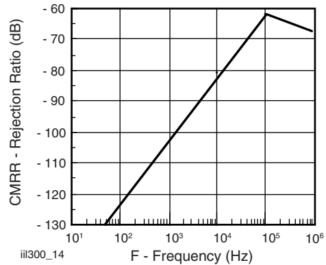
Fig. 13 - Common-Mode Rejection
