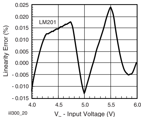
Fig. 17 - Linearity Error vs. Input Voltage
