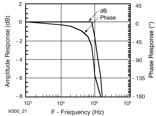
Fig. 18 - Amplitude and Phase Power Supply Control
