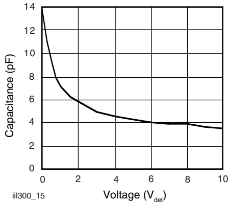
Fig. 14 - Photodiode Junction Capacitance vs. Reverse Voltage
