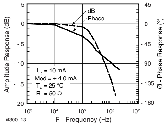
Fig. 12 - Amplitude and Phase Response vs. Frequency
