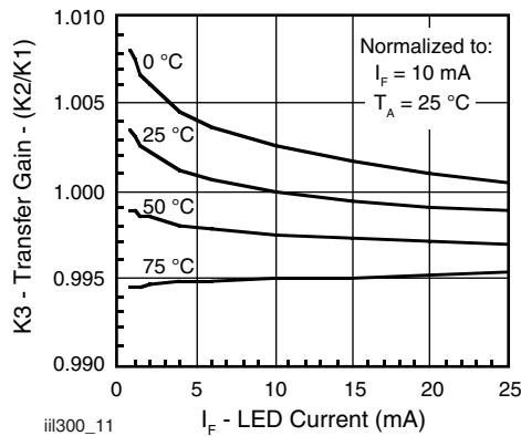
Fig. 10 - Normalized Transfer Gain vs. LED Current and Temperature
