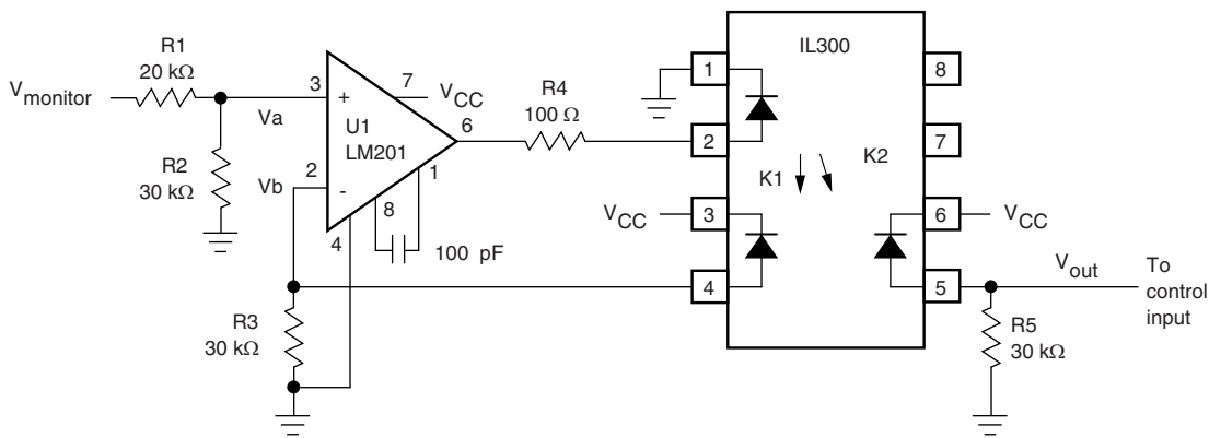
Fig. 6 - DC Coupled Power Supply Feedback Amplifier
