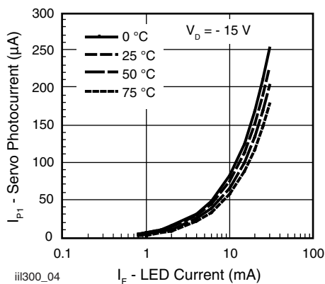
Fig. 4 - Servo Photocurrent vs. LED Current and Temperature
