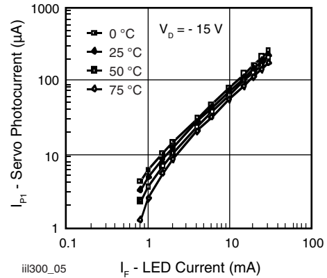
Fig. 5 - Servo Photocurrent vs. LED Current and Temperature
