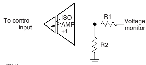
Fig. 15 - Isolated Control Amplifier
