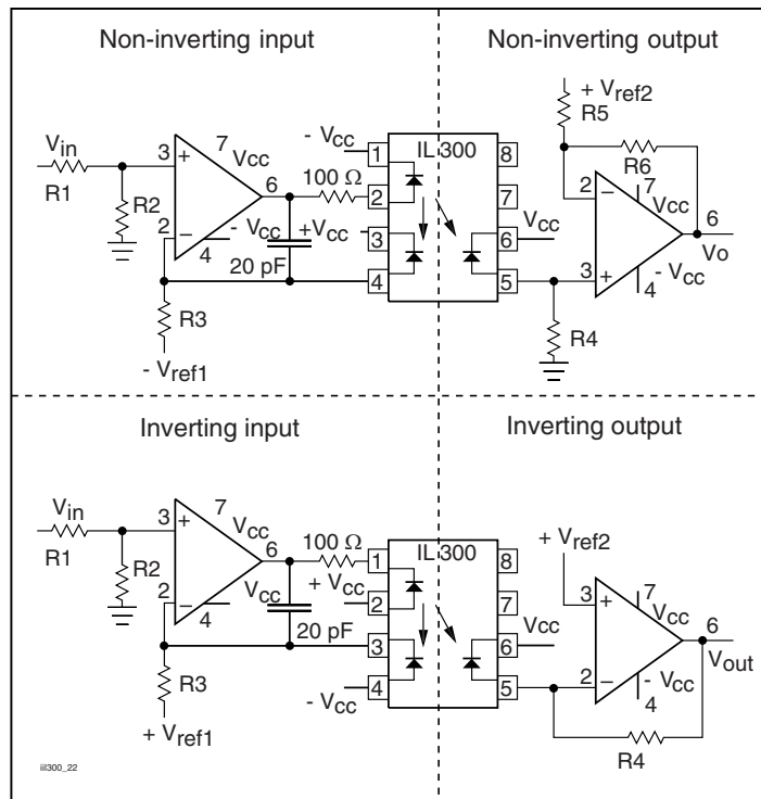
Fig. 7 - Non-inverting and Inverting Amplifiers
