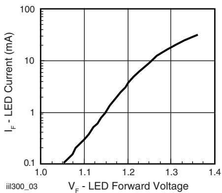
Fig. 3 - LED Forward Current vs. Forward Voltage
