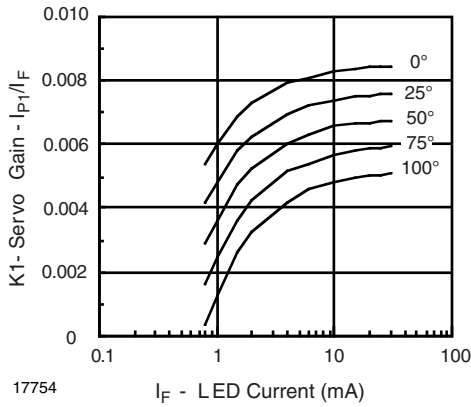
Fig. 8 - Servo Gain vs. LED Current and Temperature
