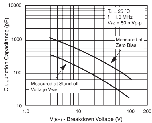
Figure 4. Typ. Junction Capacitance Uni-Directional
