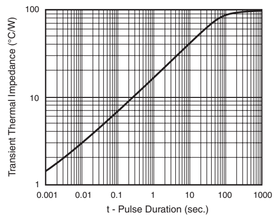
Figure 8. Typ. Transient Thermal Impedance
