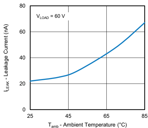
Fig. 13 - Leakage Current vs. Ambient Temperature
