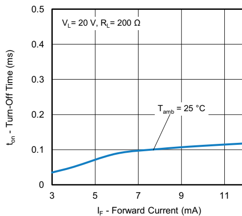
Fig. 11 - Turn-Off Time vs. Forward Current
