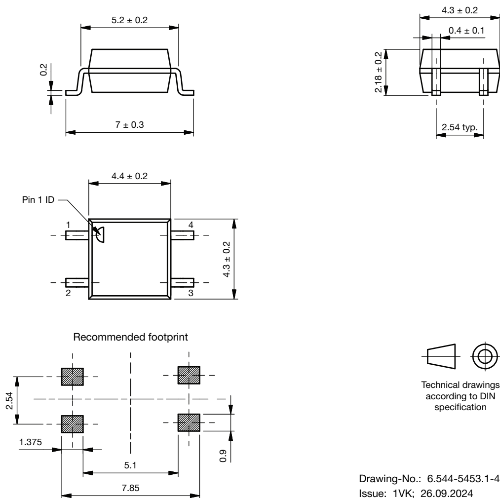
Fig. 14 - Package Drawings
