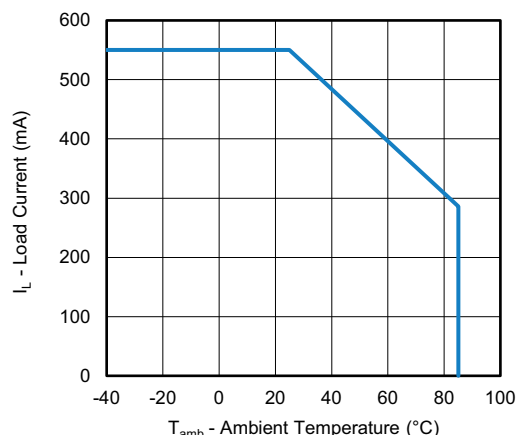
Fig. 3 - Load Current vs. Ambient Temperature
