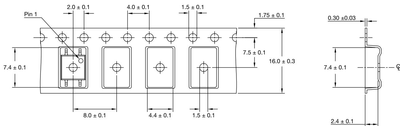
Fig. 16 - VO1400AEF (3000 pieces on reel)
