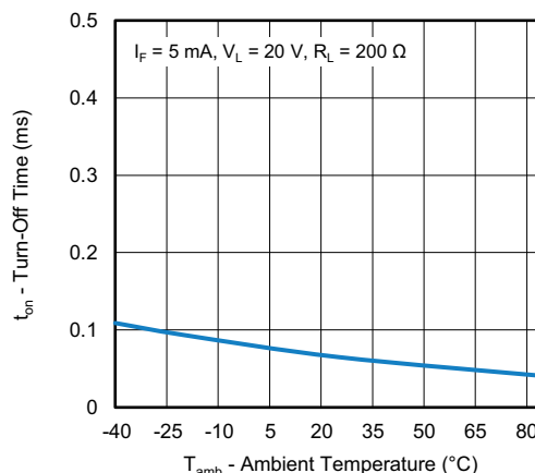
Fig. 10 - Turn-Off Time vs. Ambient Temperature
