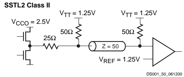
Figure 49: Terminated SSTL2 Class II
