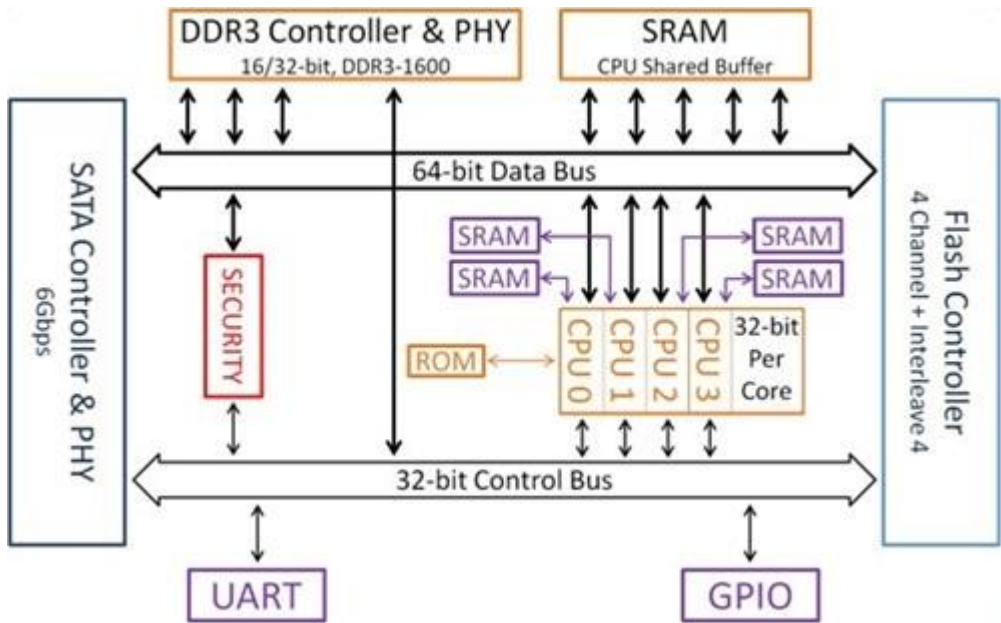
Figure 1-1 Controller Block Diagram
