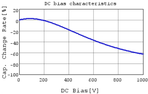
DE2E3SA472MA3BT02F C-DC bias capchange, 20.0
