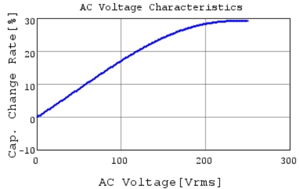
DE2E3SA472MA3BT02F C-AC Voltage capchange, I
