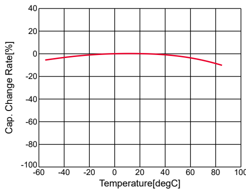
GRM155R60J154KE01#,C-Temp.,capchange, DC0.0V, AC0.5Vrms
