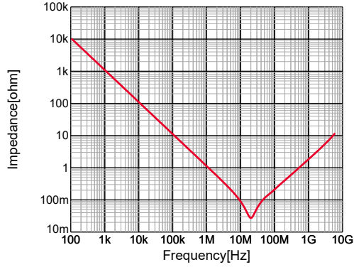
GRM155R60J154KE01#,|Z|,DC0V,25degC
