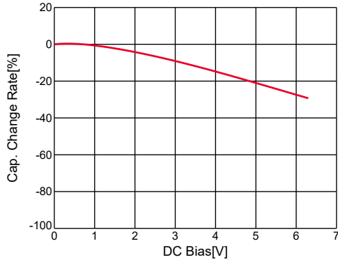
GRM155R60J154KE01#,C-DC bias,capchange, 25.0degC, AC0.5Vrms
