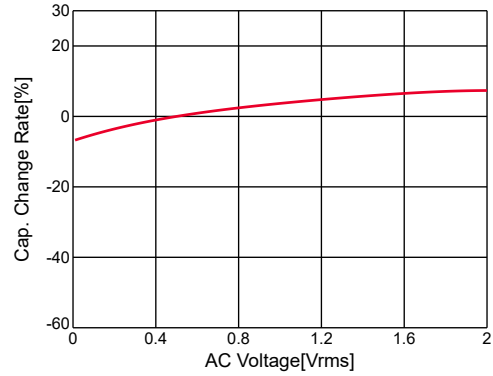
GRM155R60J154KE01#,C-AC Voltage,capchange, DC0V, 25.0degC
