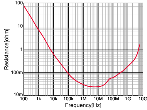
GRM155R60J154KE01#,R,DC0V,25degC
