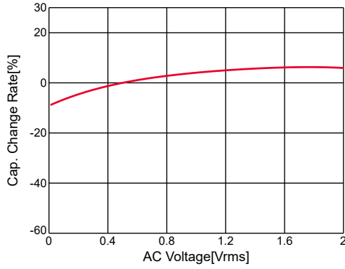
GRM155R60J824KE19#,C-AC Voltage,capchange, DC0V, 25.0degC
