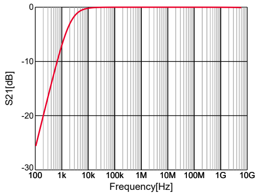
GRM155R60J824KE19#,S21,DC0V,25degC,series
