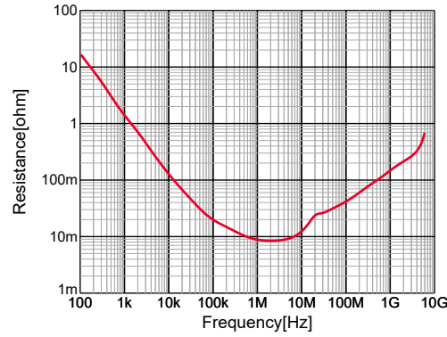
GRM155R60J824KE19#,R,DC0V,25degC
