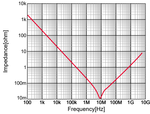
GRM155R60J824KE19#,|Z|,DC0V,25degC
