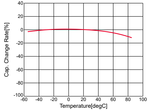
GRM155R60J824KE19#,C-Temp.,capchange, DC0.0V, AC0.5Vrms
