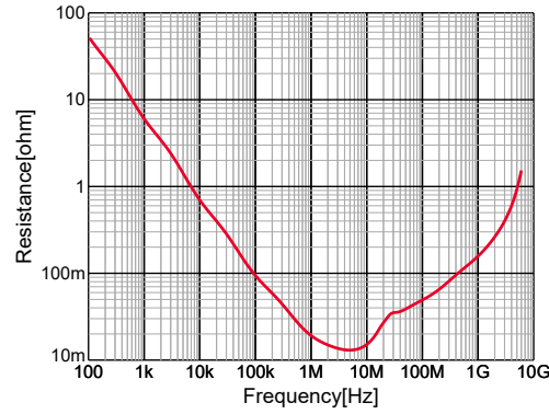
GRM185R60J105KE26#,R,DC0V,25degC
