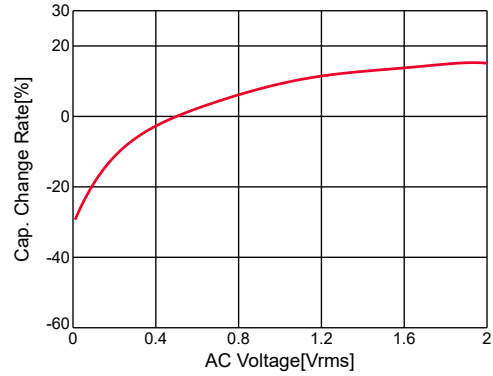
GRM185R60J105KE26#,C-AC Voltage,capchange, DC0V, 25.0degC
