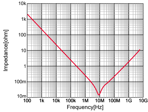
GRM185R60J105KE26#,|Z|,DC0V,25degC
