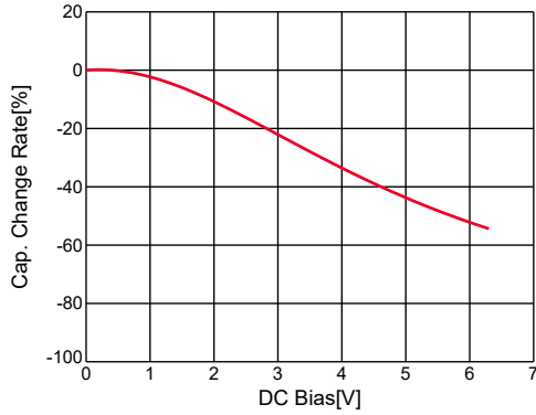
GRM185R60J105KE26#,C-DC bias,capchange, 25.0degC, AC0.5Vrms
