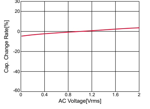
GRM188R71E224KA88#,C-AC Voltage,capchange, DC0V, 25.0degC
