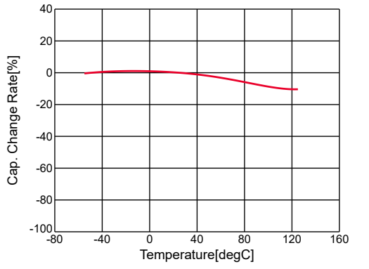
GRM188R71E224KA88#,C-Temp.,capchange, DC0.0V, AC1.0Vrms
