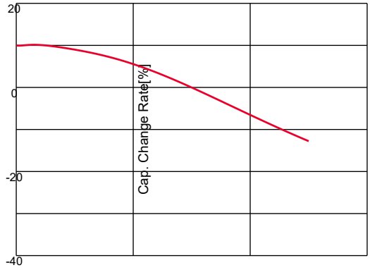
GRM188R71E224KA88#,C-DC bias,capchange, 25.0degC, AC1.0Vrms
