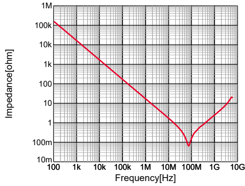
GRM188R71H103KA01#,|Z|,DC0V,25degC
