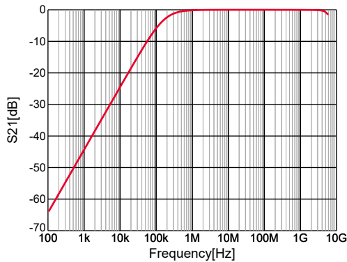
GRM188R71H103KA01#,S21,DC0V,25degC,series
