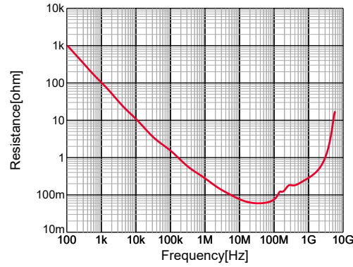
GRM188R71H103KA01#,R,DC0V,25degC
