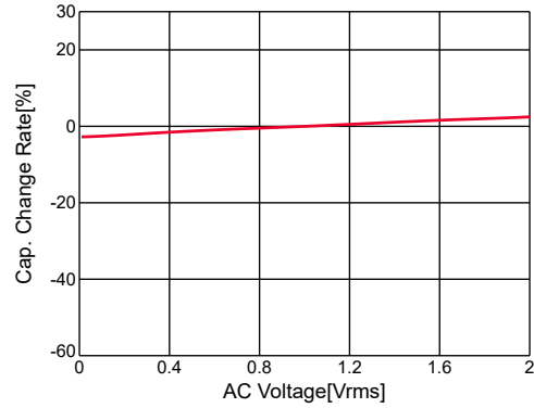
GRM188R71H104KA93#,C-AC Voltage,capchange, DC0V, 25.0degC
