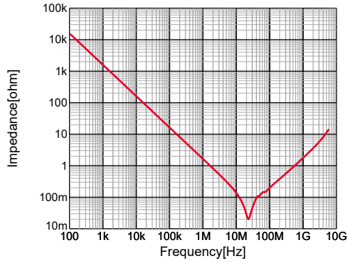
GRM188R71H104KA93#,|Z|,DC0V,25degC
