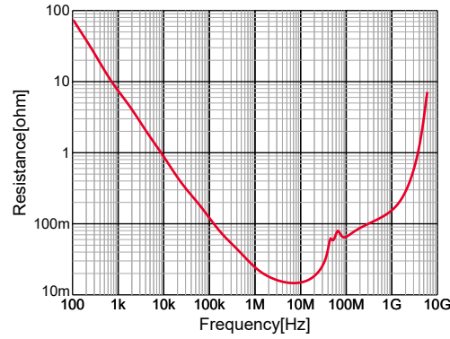
GRM188R71H104KA93#,R,DC0V,25degC
