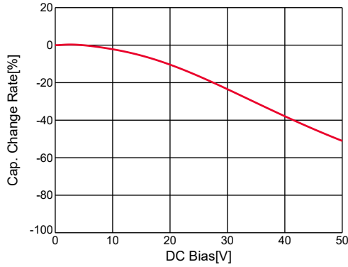
GRM188R71H104KA93#,C-DC bias,capchange, 25.0degC, AC1.0Vrms
