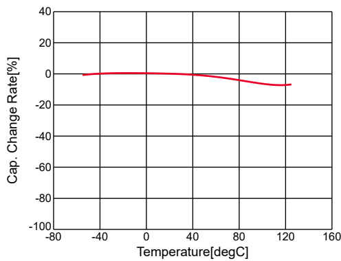
GRM188R71H104KA93#,C-Temp.,capchange, DC0.0V, AC1.0Vrms
