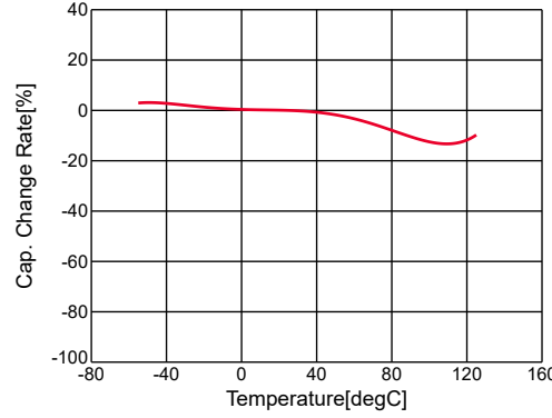
GRM21AR72D222KW01#,C-Temp.,capchange, DCOV, AC1Vrms
