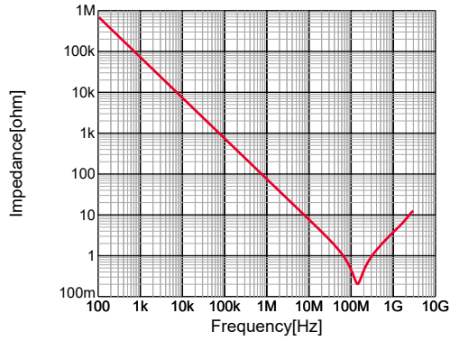
GRM21AR72D222KW01#,|Z|,DC0V,25degC
