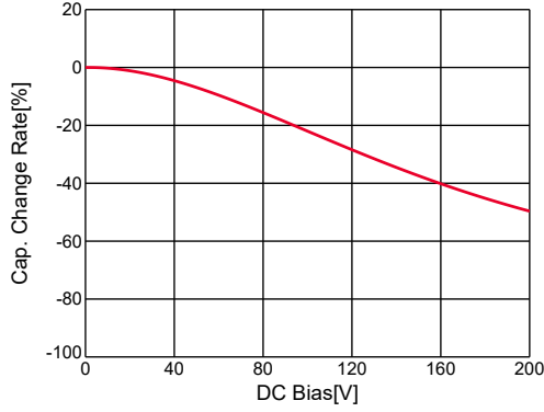
GRM21AR72D222KW01#,C-DC bias,capchange, 25.0degC, AC1Vrms
