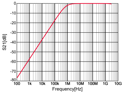
GRM21AR72D222KW01#,S21,DC0V,25degC,series
