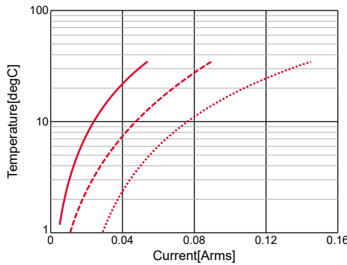
GRM21AR72D222KW01#,Temp.rise
