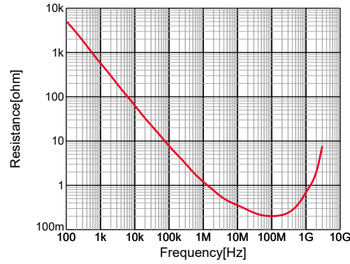
GRM21AR72D222KW01#,R,DC0V,25degC
