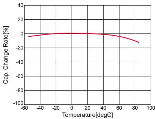
GRM21BR61A226ME51#,C-Temp.,capchange, DC0.0V, AC0.5Vrms
