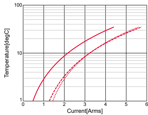
GRM21BR61A226ME51#,Temp.rise
