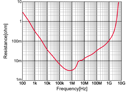
GRM21BR61A226ME51#,R,DC0V,25degC
