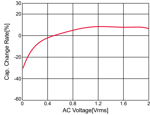
GRM21BR61A226ME51#,C-AC Voltage,capchange, DC0V, 25.0degC
