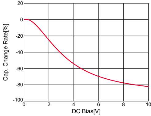
GRM21BR61A226ME51#,C-DC bias,capchange, 25.0degC, AC0.5Vrms
