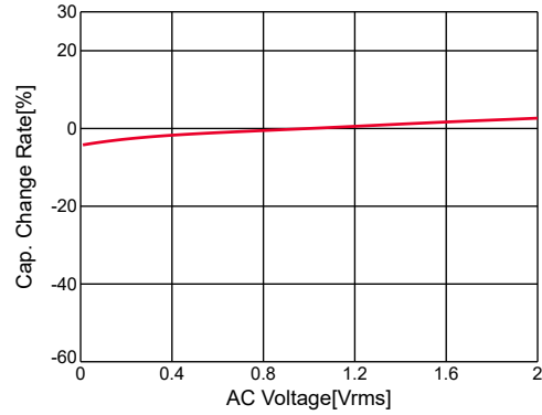
GRM21BR71C224KA01#,C-AC Voltage,capchange, DC0V, 25.0degC
