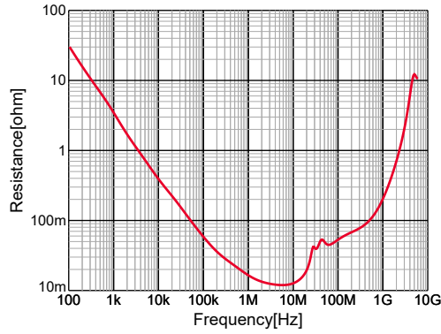
GRM21BR71C224KA01#,R,DC0V,25degC
