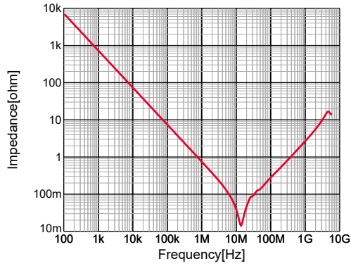
GRM21BR71C224KA01#,|Z|,DC0V,25degC
