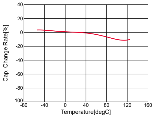
GRM21BR71C224KA01#,C-Temp.,capchange, DC0.0V, AC1.0Vrms
