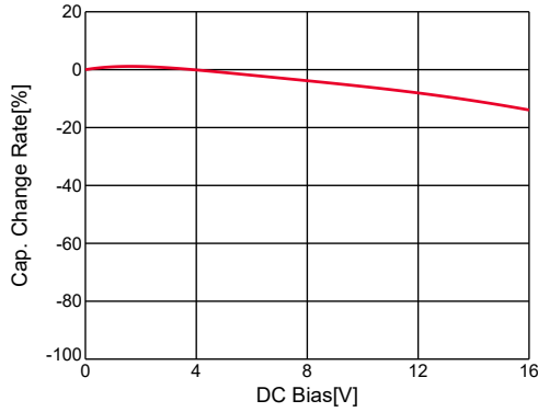
GRM21BR71C224KA01#,C-DC bias,capchange, 25.0degC, AC1.0Vrms
