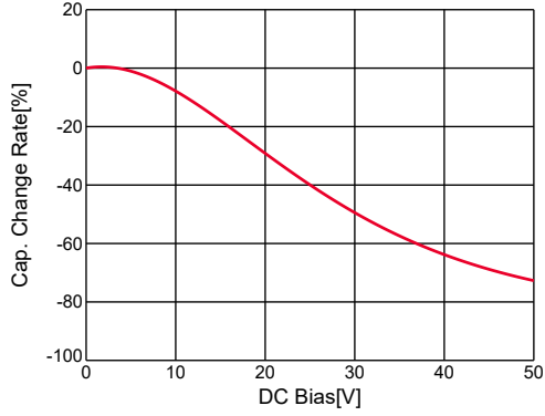
GRM21BR71H105KA12#,C-DC bias,capchange, 25.0degC, AC1Vrms
