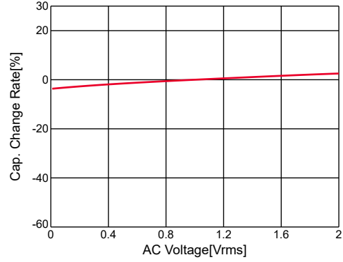
GRM21BR71H105KA12#,C-AC Voltage,capchange, DC0V, 25.0degC
