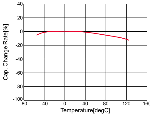
GRM21BR71H105KA12#,C-Temp.,capchange, DC0.0V, AC0.1Vrms
