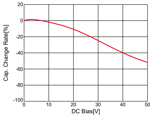
GRM21BR71H224KA01#,C-DC bias,capchange, 25.0degC, AC1.0Vrms
