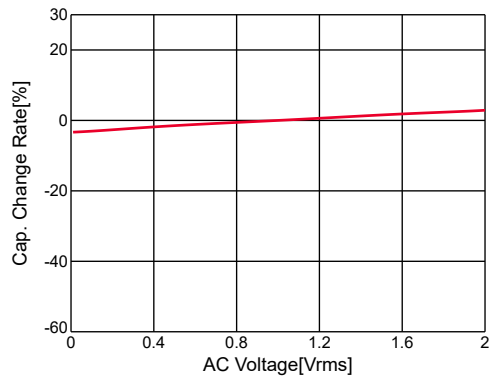
GRM21BR71H224KA01#,C-AC Voltage,capchange, DC0V, 25.0degC
