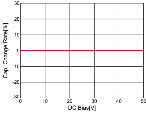
GRM31C5C1H823JA01#,C-DC bias,capchange, 25.0degC, AC1Vrms
