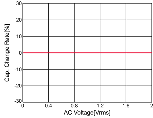
GRM31C5C1H823JA01#,C-AC Voltage,capchange, DCOV, 25.0degC
