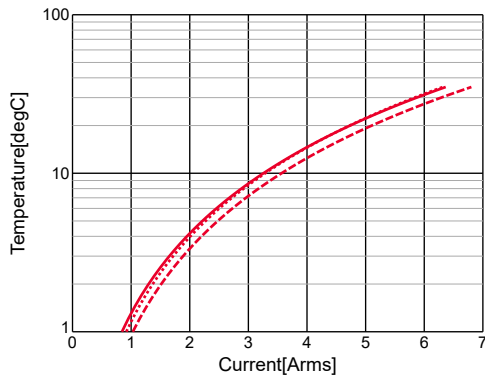
GRM31CR60J107MEA8#,Temp.rise
