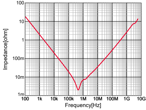
GRM31CR60J107MEA8#,|Z|,DC0V,25degC
