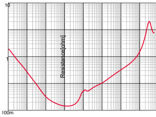
GRM31CR60J107MEA8#,R,DC0V,25degC
