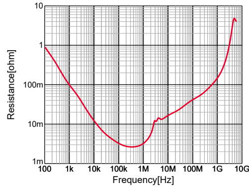
GRM31CR71C106KA12#,R,DC0V,25degC
