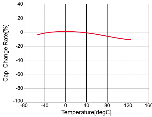
GRM31CR71C106KA12#,C-Temp.,capchange, DC0.0V, AC0.1Vrms
