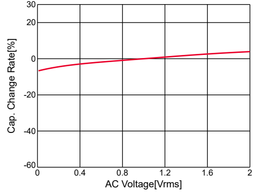
GRM31CR71C106KA12#,C-AC Voltage,capchange, DC0V, 25.0degC
