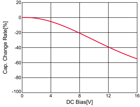
GRM31CR71C106KA12#,C-DC bias,capchange, 25.0degC, AC1Vrms
