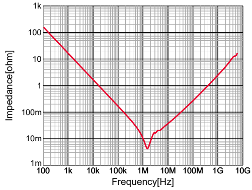
GRM31CR71C106KA12#,|Z|,DC0V,25degC
