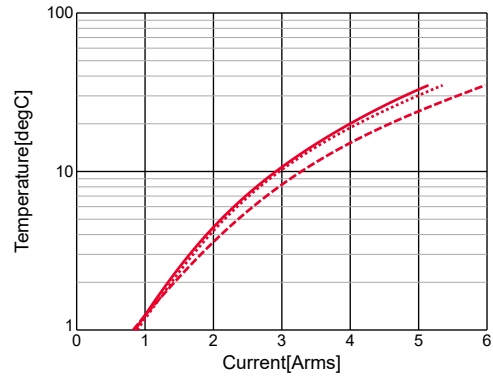
GRM31CR71C106KA12#,Temp.rise
