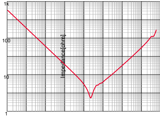
GRM31CR71E475KA88#,|Z|,DC0V,25degC
