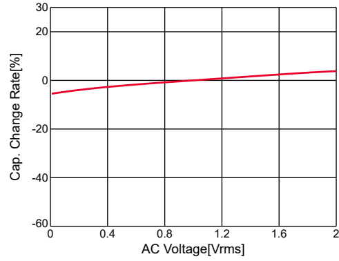
GRM31CR71E475KA88#,C-AC Voltage,capchange, DC0V, 25.0degC
