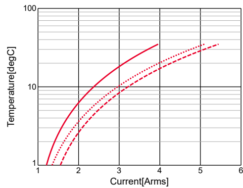
GRM31CR71E475KA88#,Temp.rise
