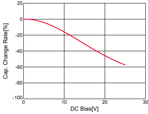
GRM31CR71E475KA88#,C-DC bias,capchange, 25.0degC, AC1Vrms
