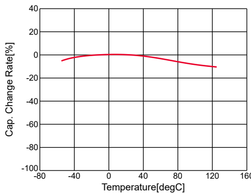
GRM31CR71E475KA88#,C-Temp.,capchange, DC0.0V, AC0.1Vrms
