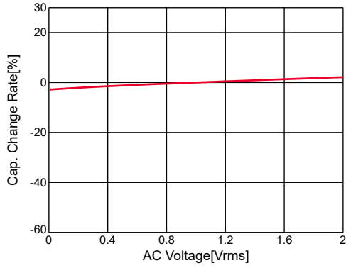
GRM31CR72A105KA01#,C-AC Voltage,capchange, DC0V, 25.0degC
