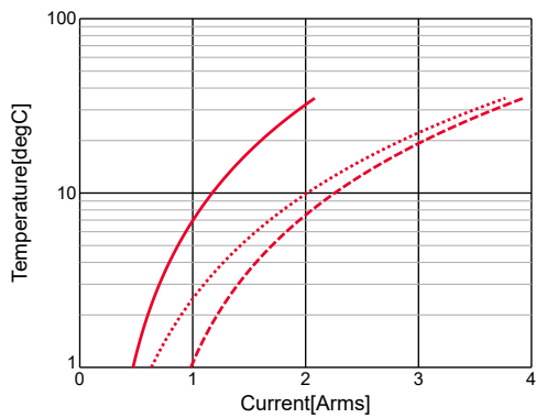
GRM31CR72A105KA01#,Temp.rise
