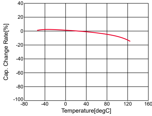
GRM31CR72A105KA01#,C-Temp.,capchange, DC0.0V, AC1.0Vrms
