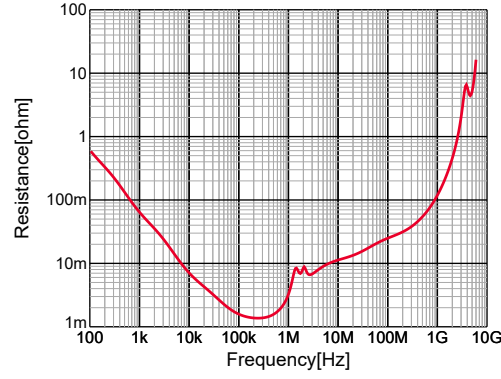
GRM32EC81C476KE15# ,R,DC0V,25degC
