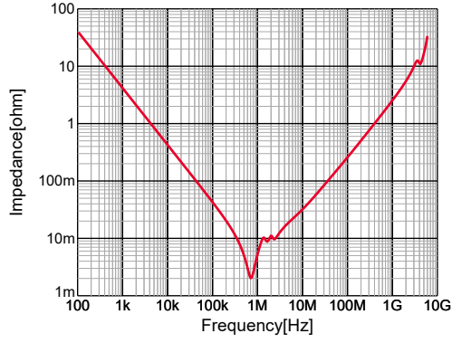
GRM32EC81C476KE15# ,|Z|,DC0V,25degC
