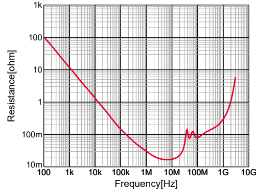
GRM43DR72J104KW01#,R,DC0V,25degC
