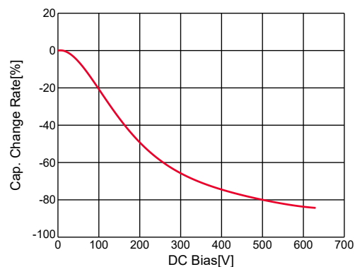
GRM43DR72J104KW01#,C-DC bias,capchange, 25.0degC, AC1Vrms
