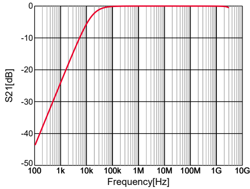
GRM43DR72J104KW01#,S21,DC0V,25degC,series
