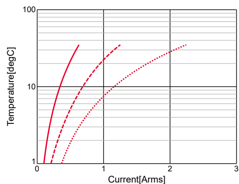
GRM43DR72J104KW01#,Temp.rise
