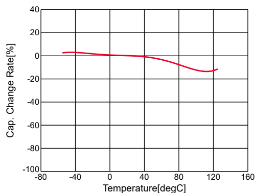
GRM43DR72J104KW01#,C-Temp.,capchange, DCOV, AC1Vrms
