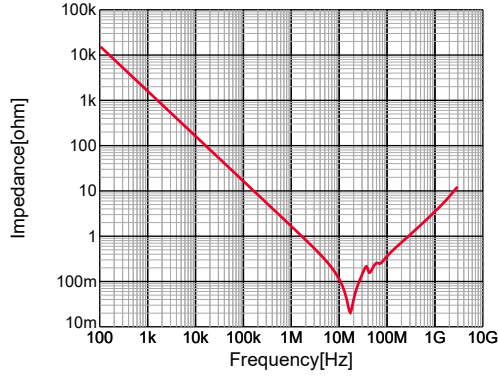
GRM43DR72J104KW01#,|Z|,DC0V,25degC
