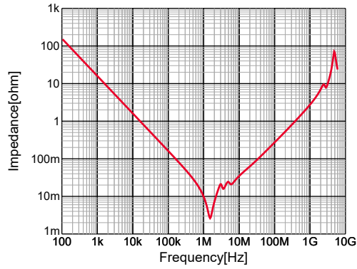
GRM55DR61H106KA88#,|Z|,DC0V,25degC
