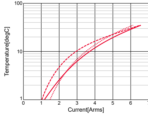
GRM55DR61H106KA88#,Temp.rise
