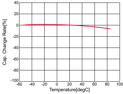
GRM55DR61H106KA88#,C-Temp.,capchange, DC0.0V, AC1.0Vrms
