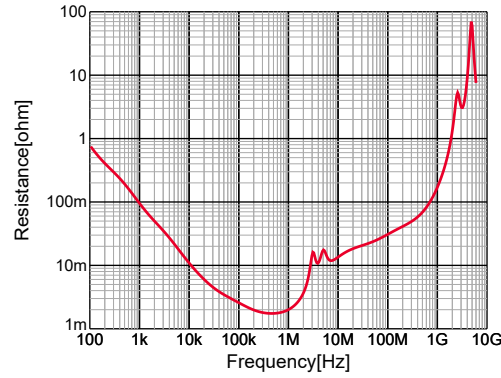
GRM55DR61H106KA88#,R,DC0V,25degC
