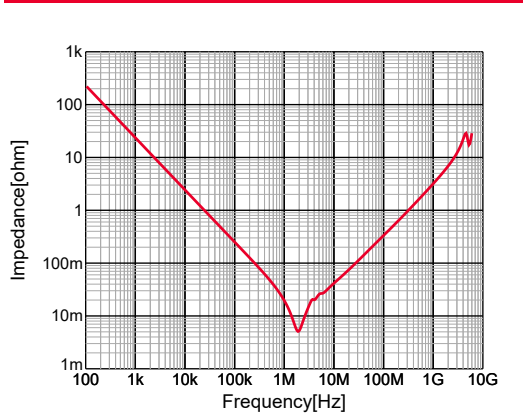
GRT31CR61H106KE01#,|Z|,DC0V,25degC
