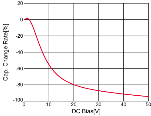
GRT31CR61H106KE01#,C-DC bias,capchange, 25.0degC, AC1.0Vrms
