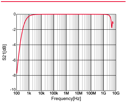
GRT31CR61H106KE01#,S21,DC0V,25degC,series
