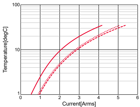
GRT31CR61H106KE01#,Temp.rise
